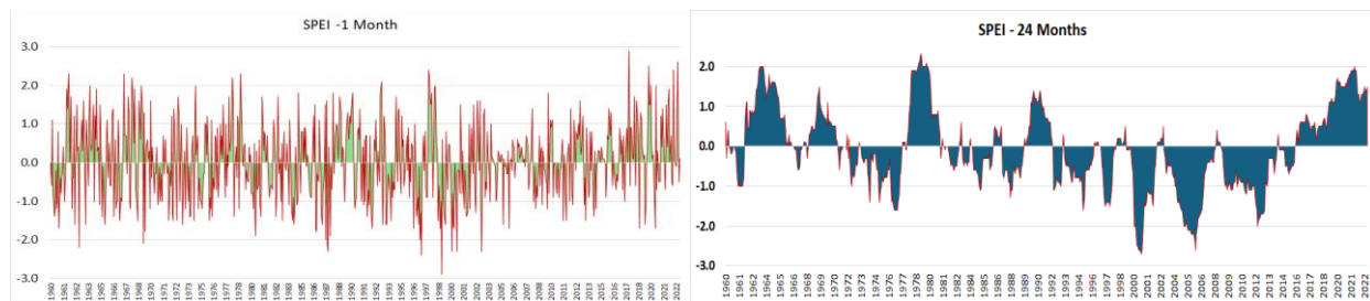
Figure 3: Standard Precipitation and Evapotranspiration Index (SPEI) for Kajiado analyzed for one month and 24 months, respectively.
